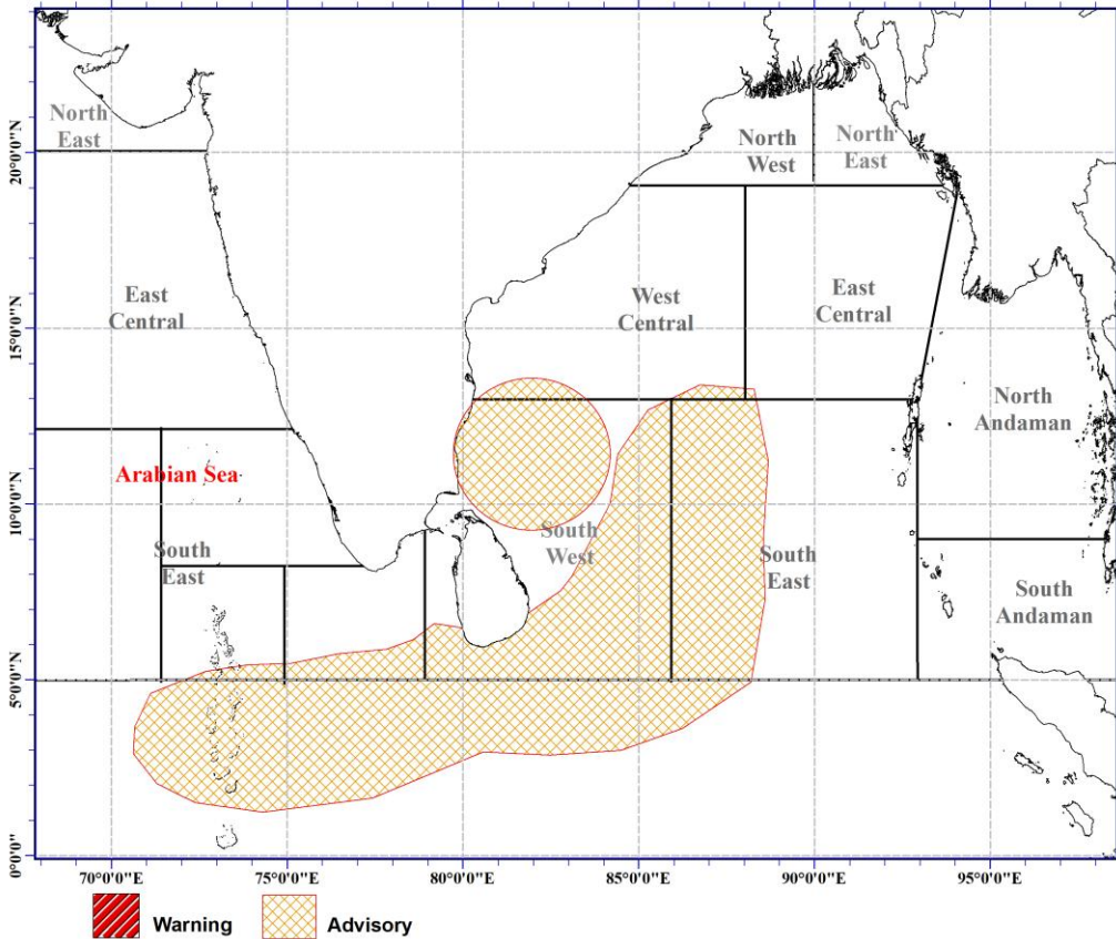
Advisory for low pressure area over Southwest Bay of Bengal. Issued at 03.00 p.m. on 13 May 2026 for the period until 03.00 p.m. 14 May 2026.
