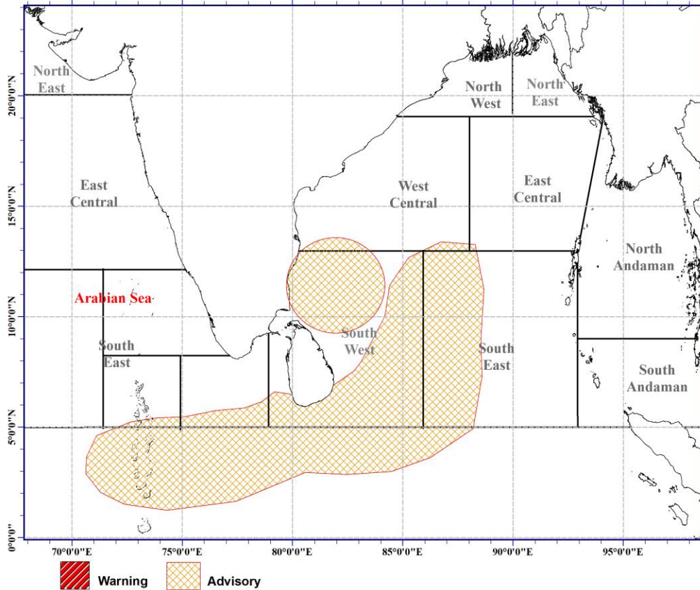
Location of the low-pressure area in the Southwest Bay of Bengal
