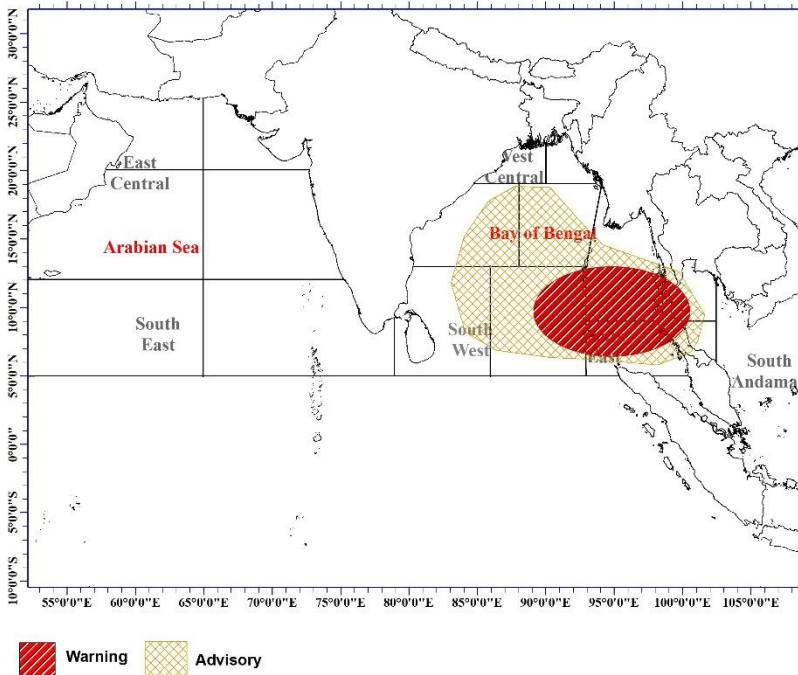
Advisory for the low pressure area issued at 04.00 p.m. on 01 December 2021 valid for next 24 hours
